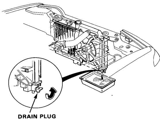
DRAIN PLUG
